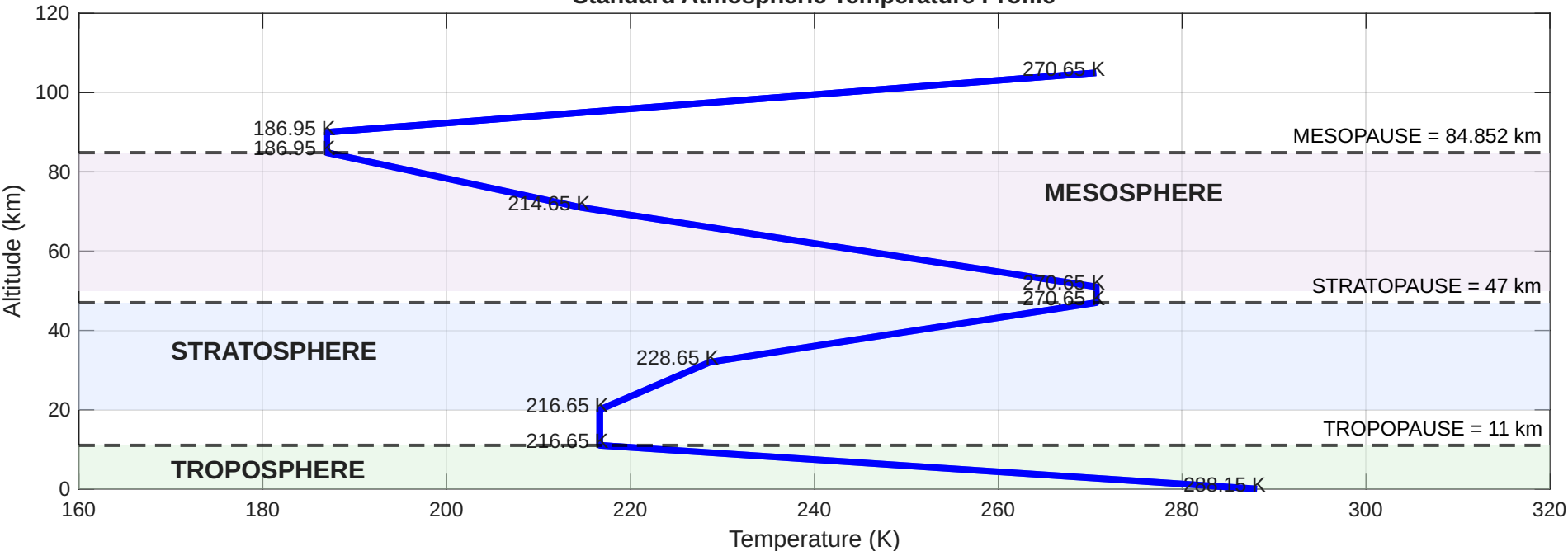
Standard Atmospheric Temperature Profile
